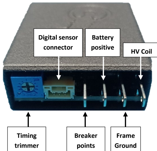
Figure 1: Front view
