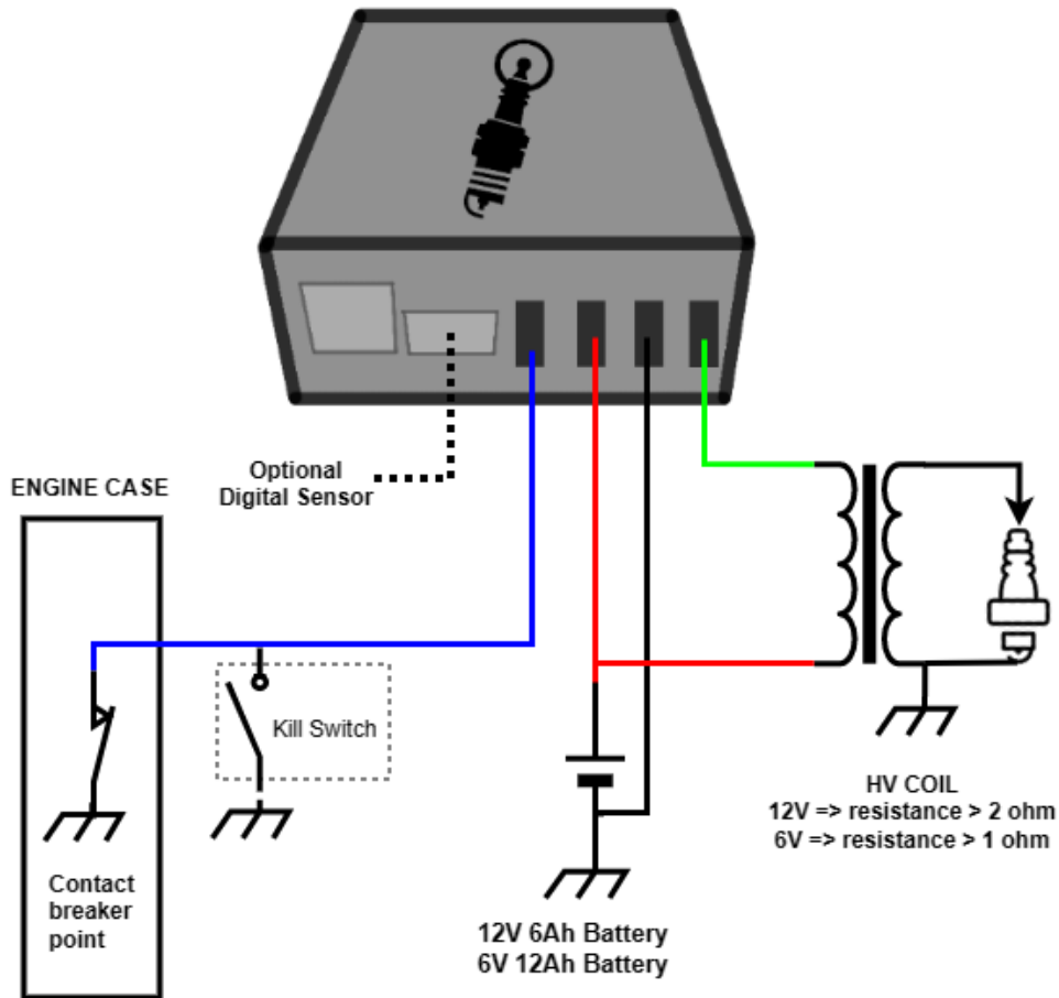
Figure 2: Electrical connection diagram
